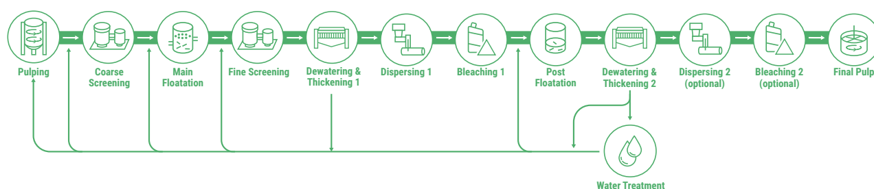
Figure 22 Typical deinking process
