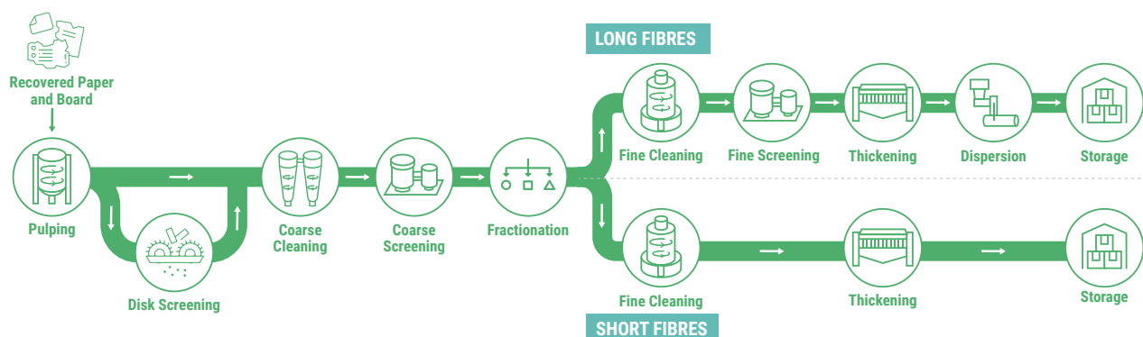
Figure 21 Typical recycling process using packaging or mixed paper
